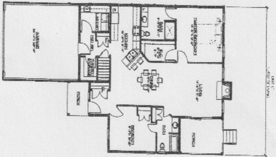
UNIT 'C' FIRST FLOOR PLAN N.T.S. 1,202 SF LIVING 176 SF PORCHES 441 SF GARAGE
