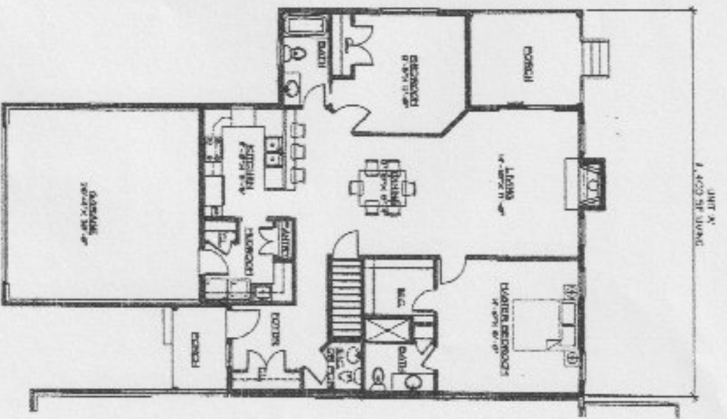
UNIT 'A' FIRST FLOOR PLAN
